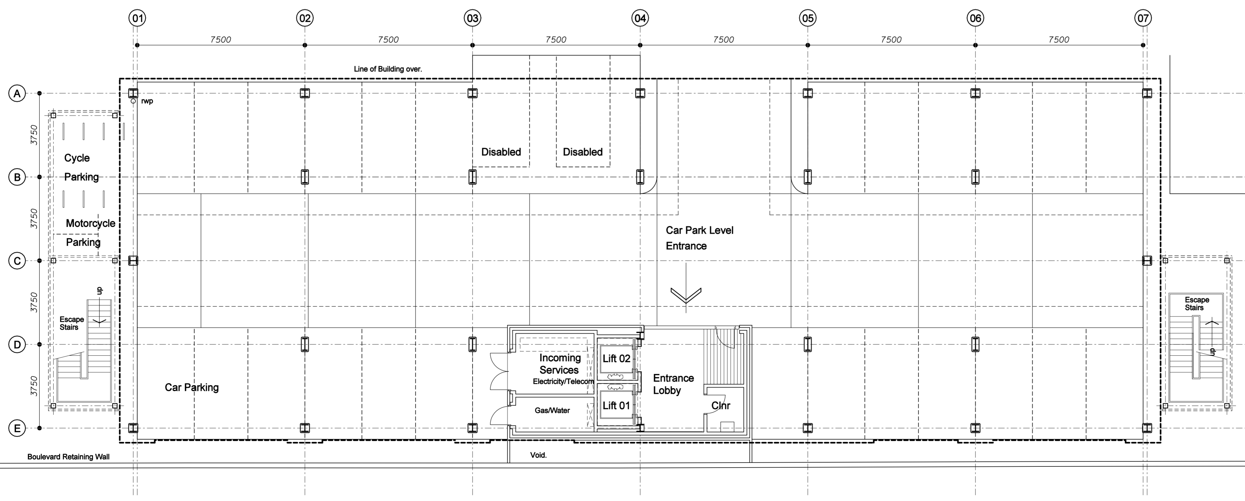
OFFICE B - CAR PARK LEVEL 04080 - 110 SCALE 1:100
