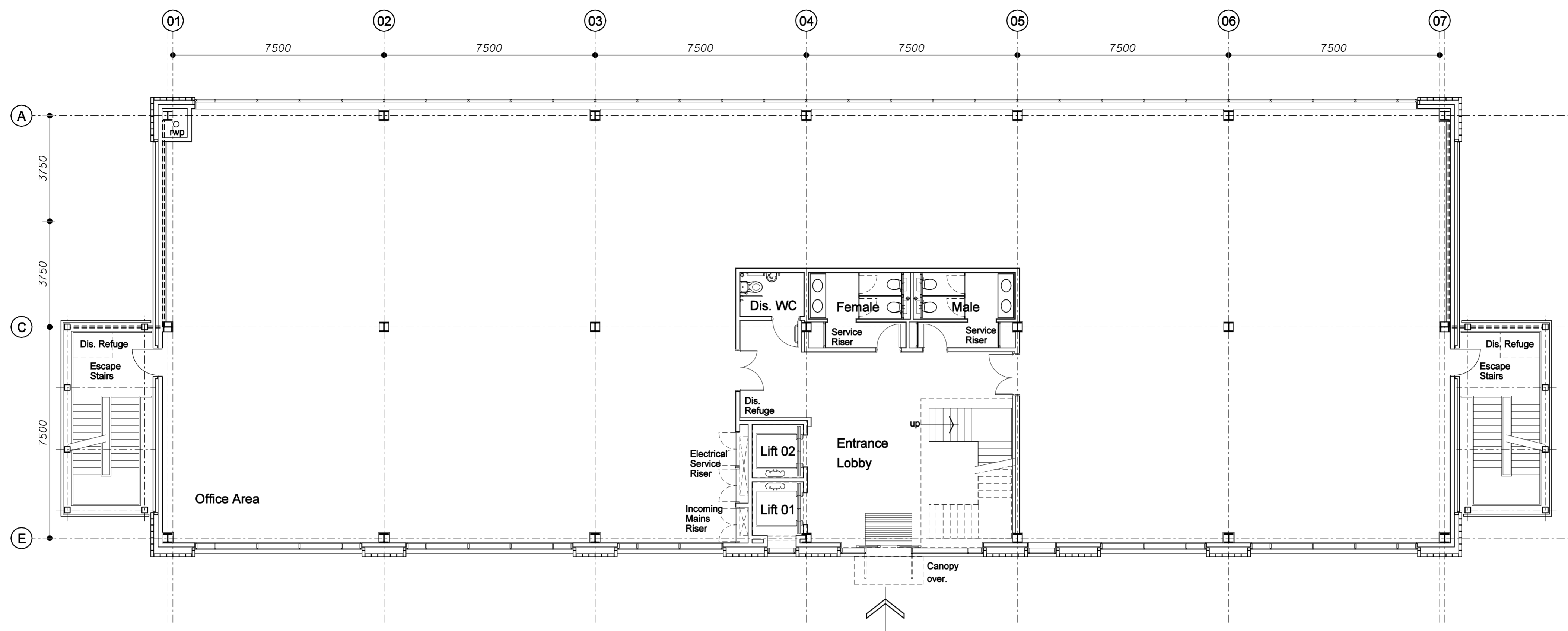
OFFICE B - LEVEL 0 04080 - 110 SCALE 1:100
